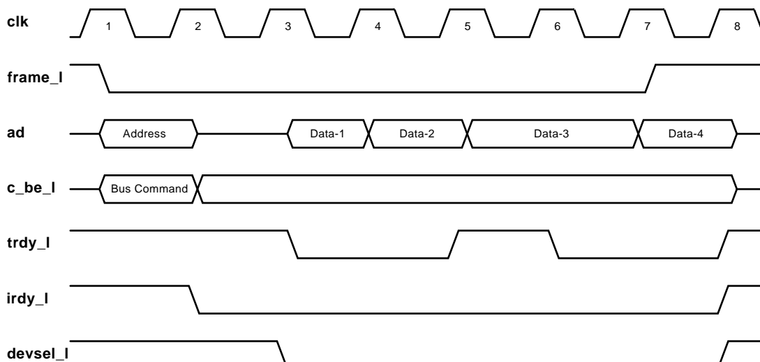
Figure 5–5 Memory Read Cycle
